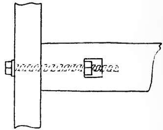
DRAW BOLT JOINT
